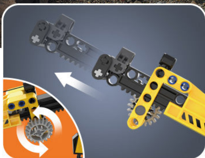
Boom extension
